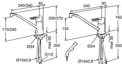
41208255 10; 41209295 10 with shut-off 41109252 with brush
