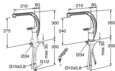
41208355; 41208395 with shut-off 41108352 with brush
